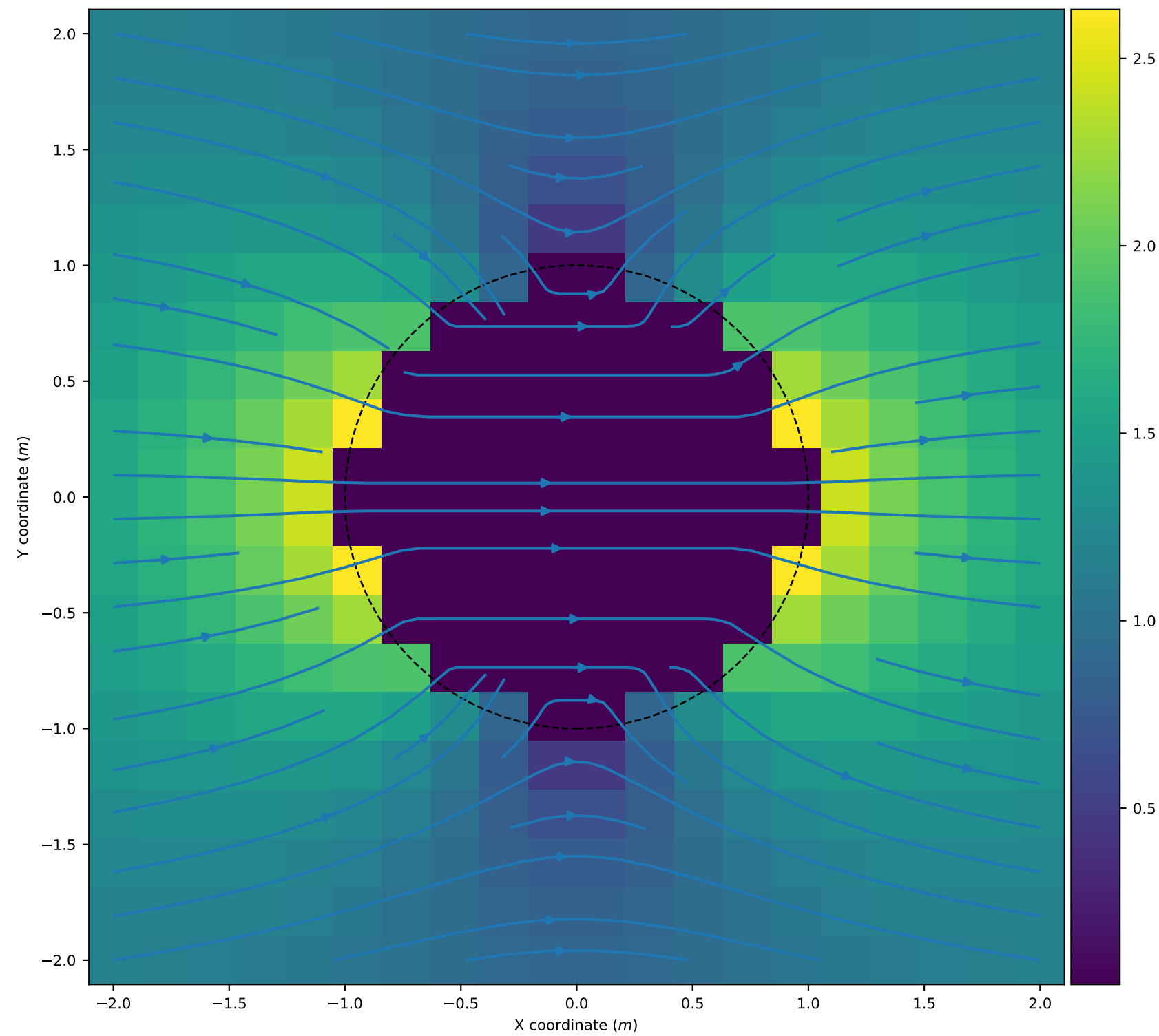
Total Electric Field
