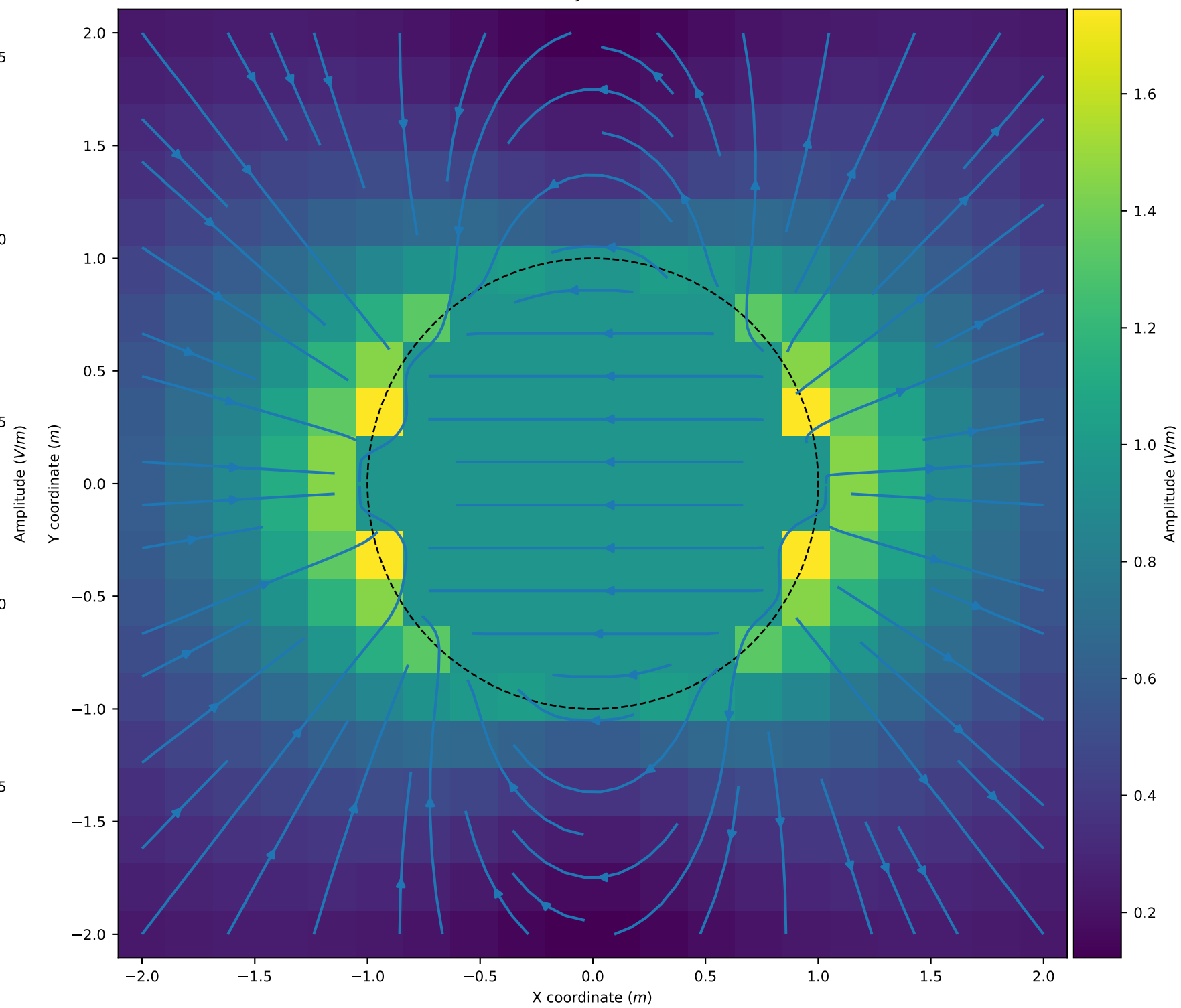
Secondary Electric Field
