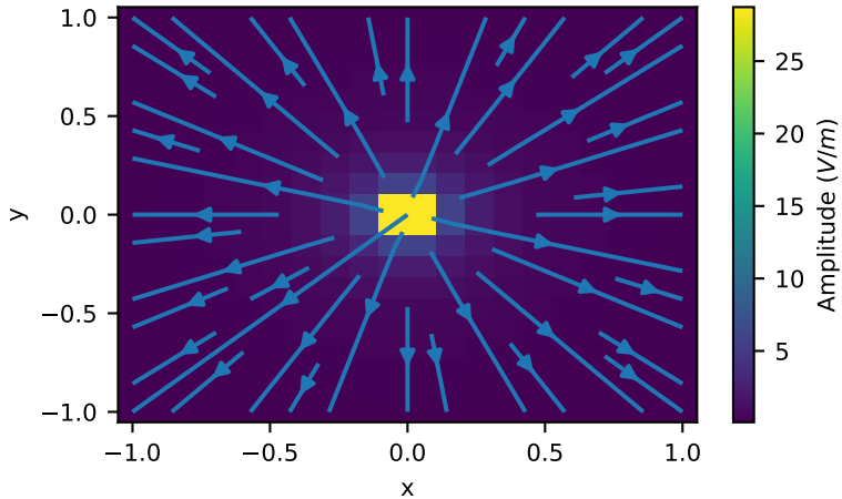
Electric Field Lines for a Point Current in a Halfspace
