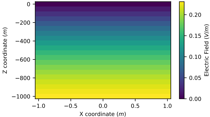
Electric Field of a Transient Planewave in the x-direction in a Wholespace
