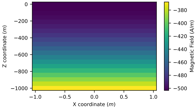
Magnetic Field of a Transient Planewave in the x-direction in a Wholespace
