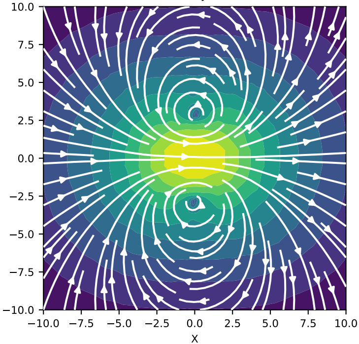
Current density at 1e-06 s
