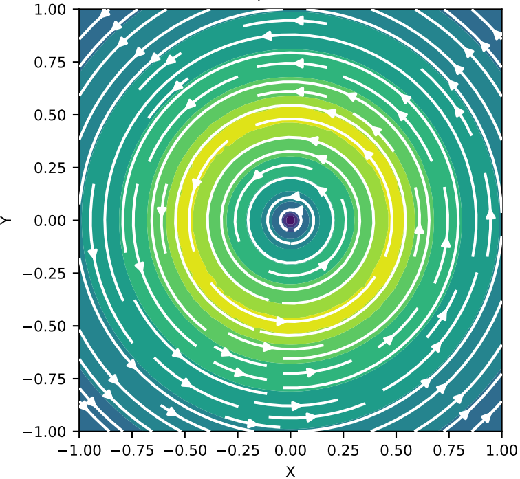
Vector potential at z=0
