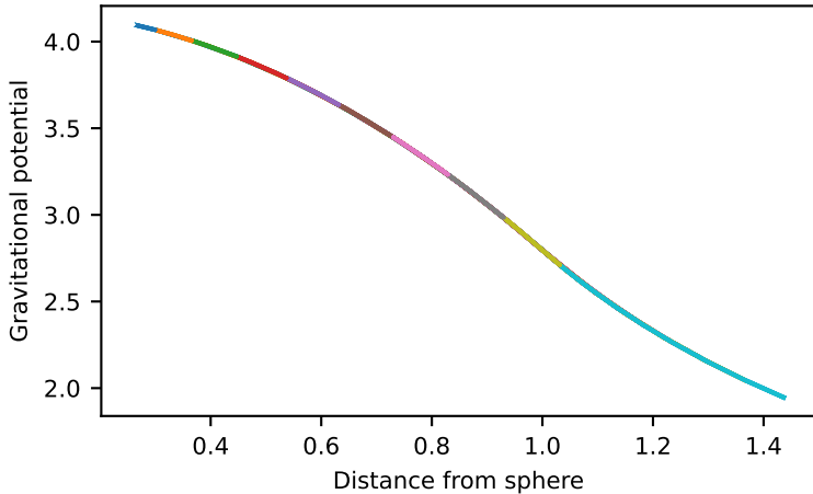
Gravitational Potential as a function of distance from sphere 1e-10
