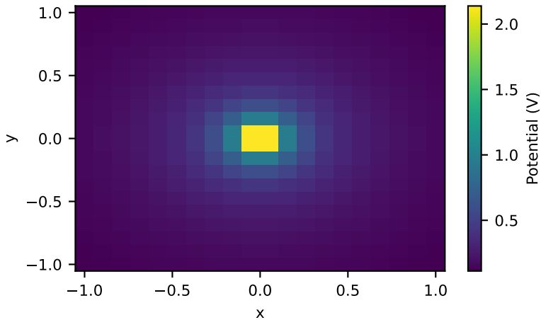
Electric Potential from Point Current in a Halfspace
