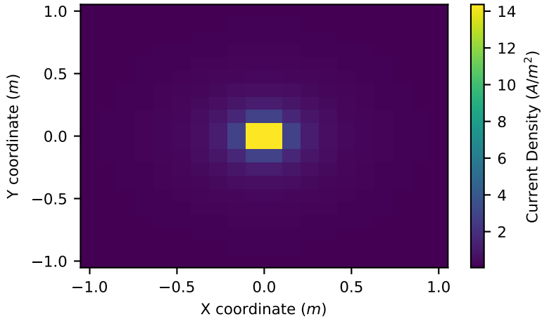
Current Density for a Point Current in a Wholespace
