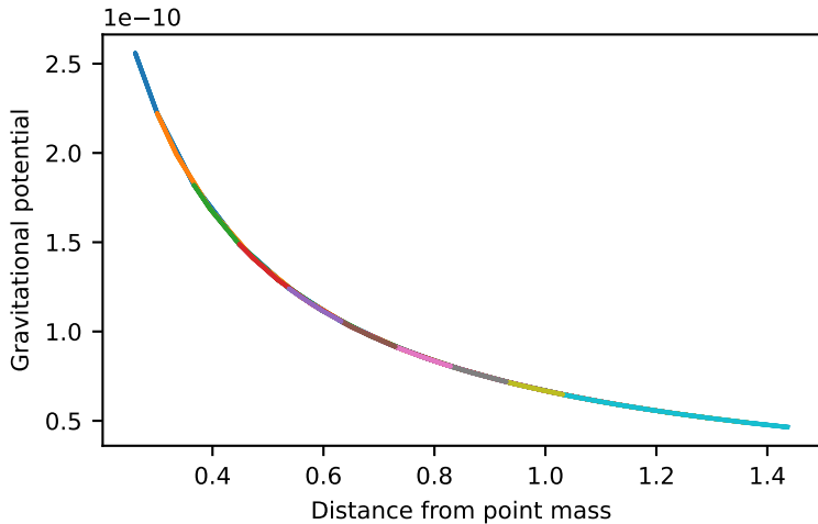
Gravitational Potential as a function of distance from point mass
