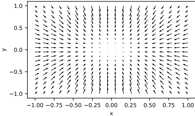
Gravitational Field Lines for a Sphere
