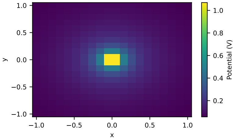
Electric Potential from Point Current in a Wholespace
