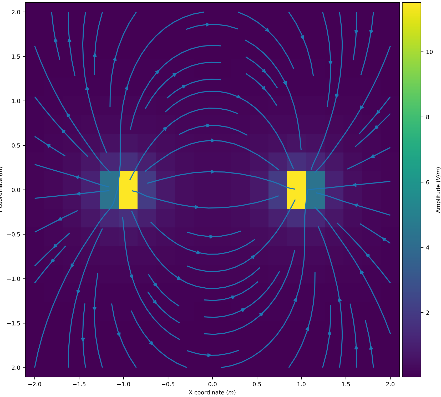
3 Electrodes
