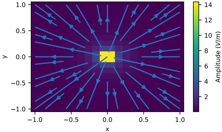
Electric Field Lines for a Point Current in a Wholespace
