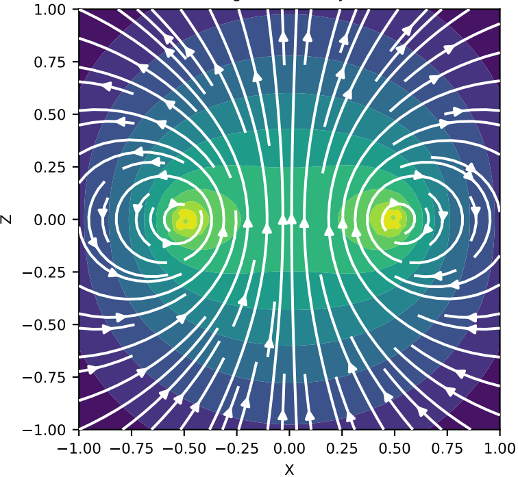
Magnetic field at y=0
