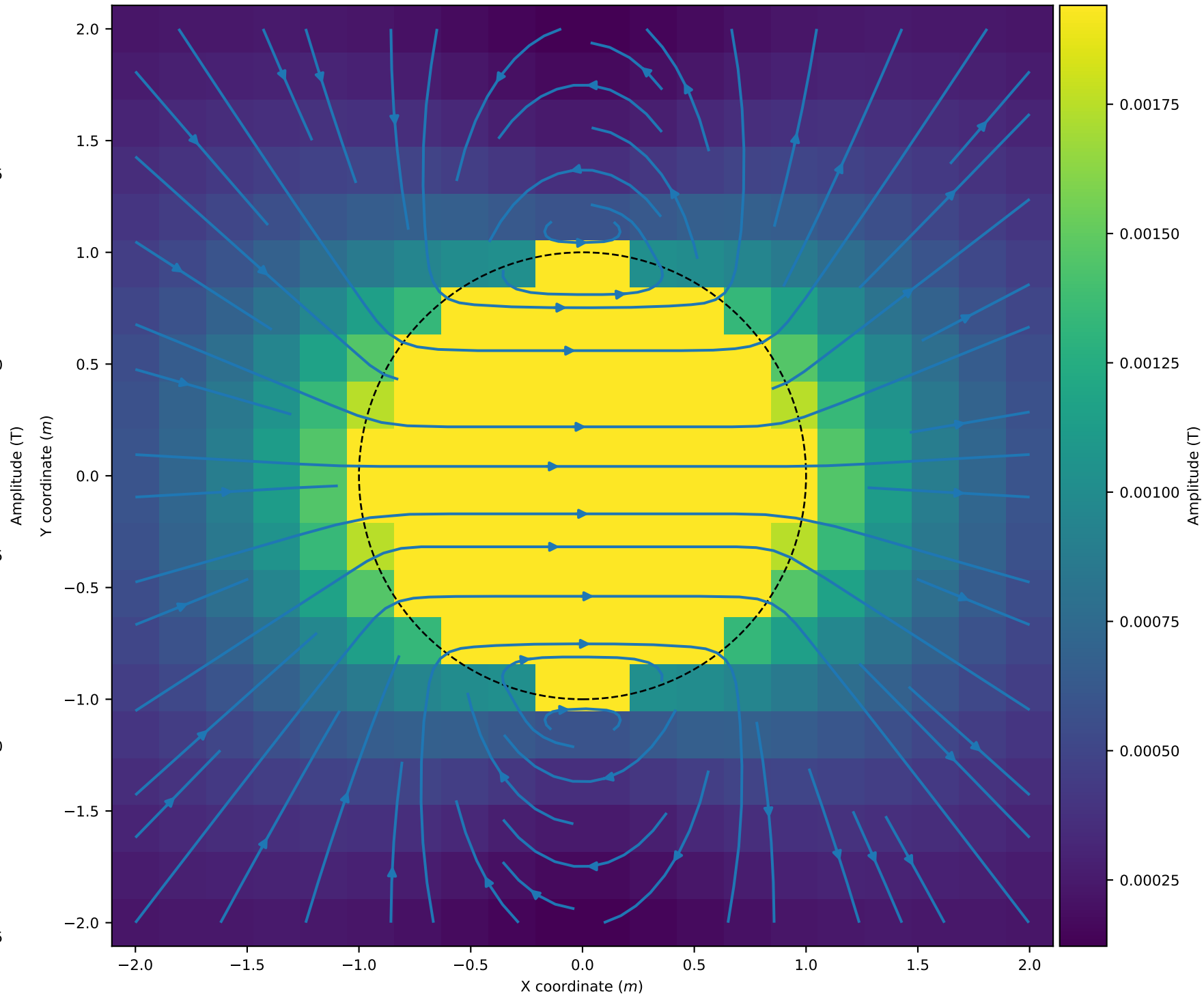
Secondary Magnetic Flux Density
