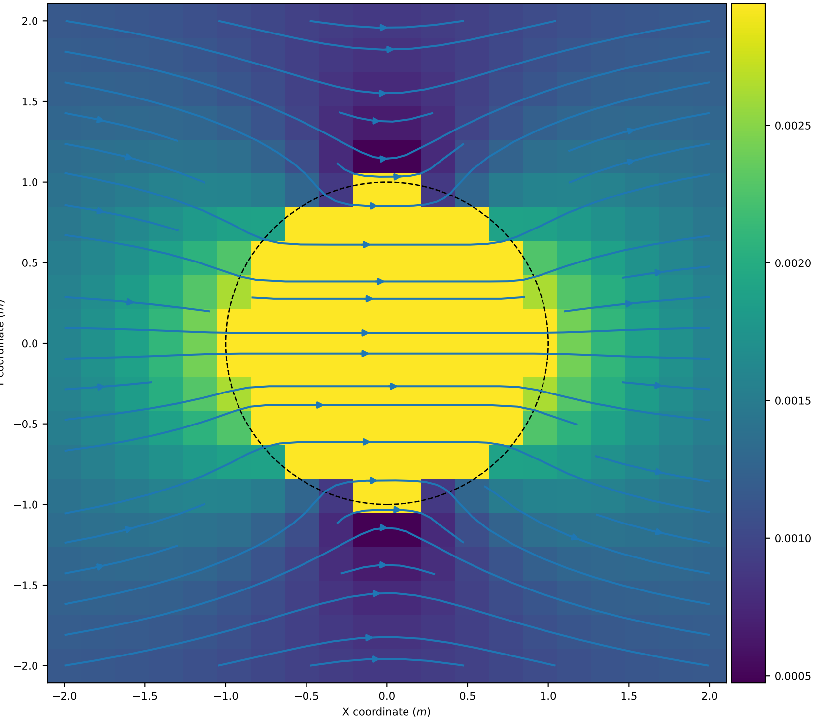
Total Magnetic Flux Density
