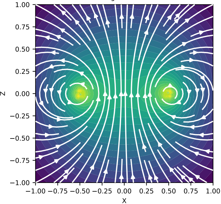
Magnetic field
