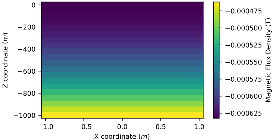
Magnetic Flux Density of a Transient Planewave in the x-direction in a Wholespace
